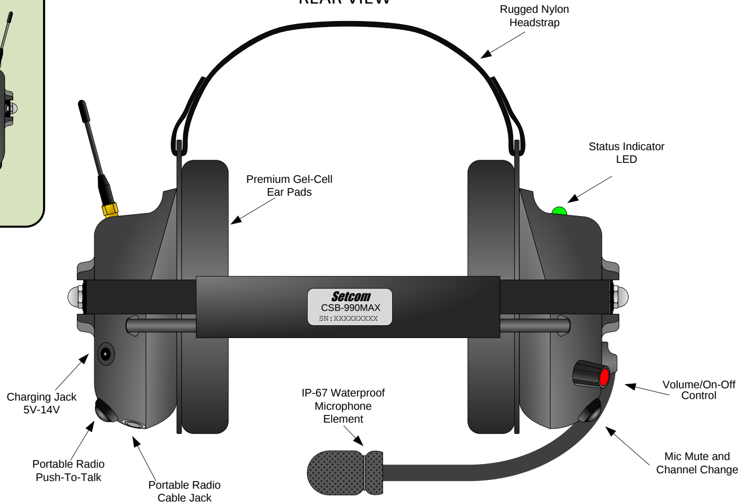
REAR VIEW
