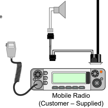
RC-18 Radio Interface Cable
